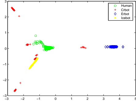
Figure 2: Data representation after dimension reduction by Isomap, where a point represents a trace of a human user (green circle) or from a bot (others). The x- and y-axes are the first and second principal coordinates [6] from Isomap. As the figure shows, the human data and the bot data are well separated. Classification in this space using k NN or SVM (or SSVM) can be performed with a high degree of accuracy.
