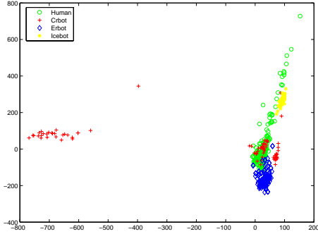
Figure 3: Dimension reduction by PCA, where the x- and y-axes represent the first and second principal components respectively. The points of human users and bots overlap, so they are not as distinguishable from each other as the result obtained by Isomap.
