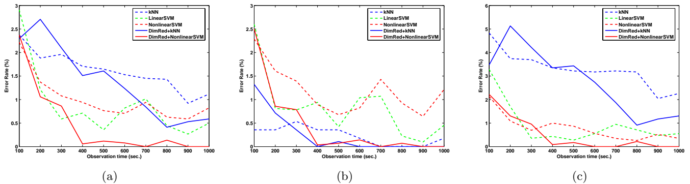
Figure 4: The error rates with different trajectory observation times, measured in seconds: (a) error rate, (b) false positive rates, and (c) false negative rates. The results are similar to those given in the previous section: 1) the methods combined with Isomap outperforms those without it; and 2) the methods based on SSVM outperform those based on k NN, except those with false positive rates.
